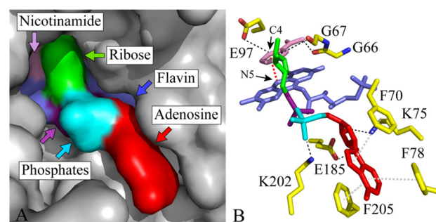
Figure 3. Occlusion of the flavin by the binding of adenosine, AMP, ADP, ADP-ribose, and NAD(H). (A) NAD(H)-bound active site in complex I from Thermus thermophilus (Protein Data Bank entry 3IAM 5 ) in surface representation. The bound NAD(H) molecule is colored with the adenosine moiety (including the second ribose) in red, the two phosphates in cyan and purple, the first ribose in green, and the nicotinamide in pink. The flavin is colored blue, and the protein is colored gray. (B) The flavin and bound nucleotide are shown as sticks from the same viewpoint, using the same color scheme. Amino acids that interact with the bound nucleotide are colored yellow, with hydrogen bonding interactions shown by dashed black lines, hydrophobic stacking interactions by dashed gray lines, and the hydride transfer between C4 of the nicotinamide ring and N5 of the flavin isoalloxazine ring by a dashed red line.
